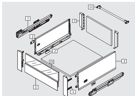
Front Section, Glass front and Rod for Push-open Synchronization not included in the Kit
